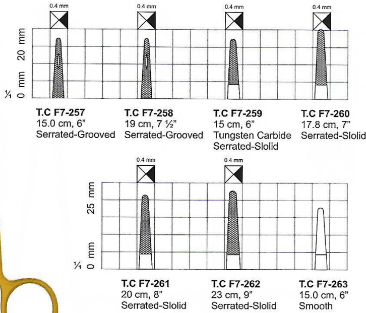
Crile-Wood Needle Holders T.C
