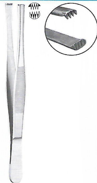
Tissue Forceps 4x5 Teeth F5-106 11.4 cm 4 1/2" F5-107 12.7 cm 5" F5-108 14 cm 5 1/2" F5-109 15.9 cm 6 1/4" F5-110 17.8 cm 7" F5-111 20.3 cm 8" F5-112 25.4 cm 10" F5-113 30.5 cm 12"
